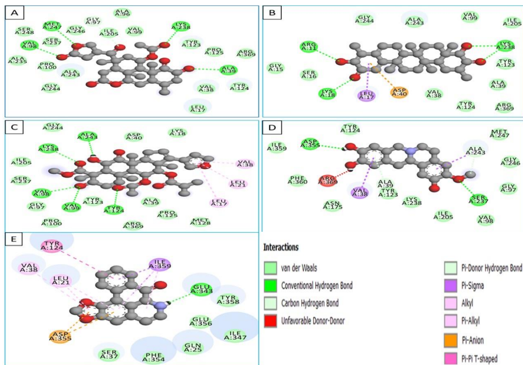
Figure 2 2D interaction of interacting residues of Cystalyzin with A) ZINC000069482017, B) ZINC000066112069, C) ZINC000069481898, D) ZINC00006017795, and E) ZINC000000006256. Different types of interaction are displayed by different colors
