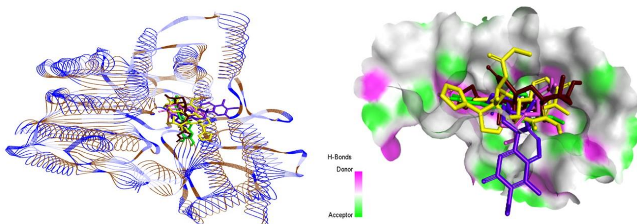
Figure 1 3D representation of Cystalyisin interacting with top five screened compounds.
