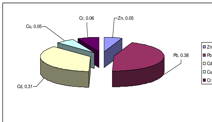
Figure 3A Relative distribution of heavy metals in water in different
