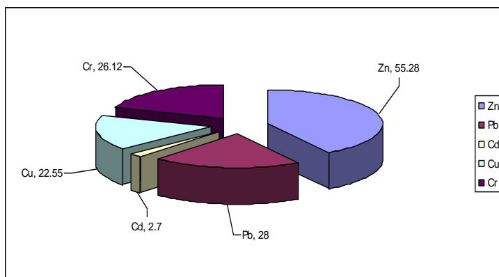
Figure 3B Relative distribution of heavy metals in Soil in different studied stations during 2010
